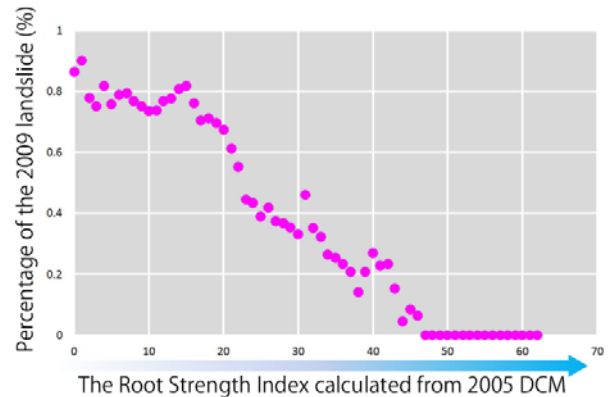
Fig. 8 Percentage of the landslides that occurred during the 2009 heavy rainfall in the Hofu region, in comparison with the root strength index calculated from 2005 LiDAR DCM.
