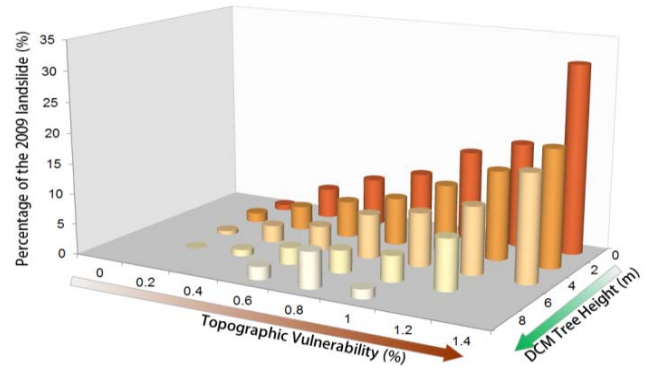
Fig. 7 Percentage of the 2009 landslides in the Hofu region, the topographic vulnerability, and the tree height derived from the 2005 LiDAR DCM. The data were summarized in 30-m grid, and the data sections less than 100 cells were omitted.
