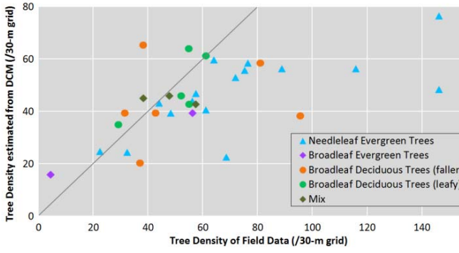
Fig. 6 The tree densities estimated from 1-m DCM and measured data in the fields.
