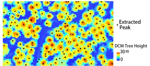
Fig. 5 An example of extracted peaks (black dots) using 3 \times 3 maximum filter from 1-m DCM of a Japanese cedar forest in the Shobara region.
