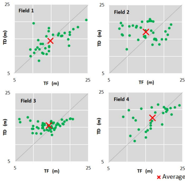
Fig. 4 Individual tree height for broadleaf deciduous forests in the Izumozaki region (green dots). TF: Tree height of field data, TD: Tree height estimated from corrected 1-m DCM.
