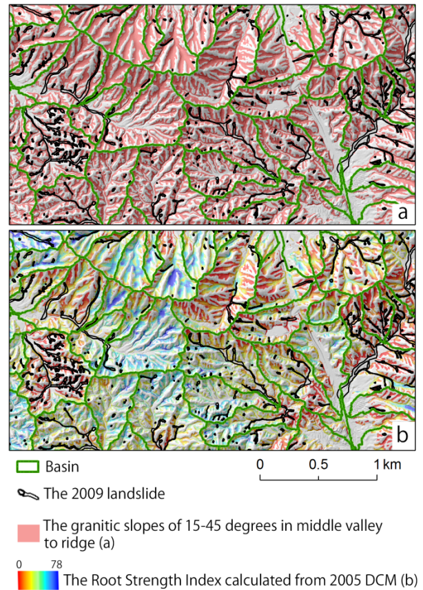
Fig. 9 The granitic slopes of 15 to 45 degrees in middle valley to ridge in a part of the Hofu area (a), and the root strength index added to the object areas (b), in comparison with the 2009 landslide and basins calculated from DEM.
