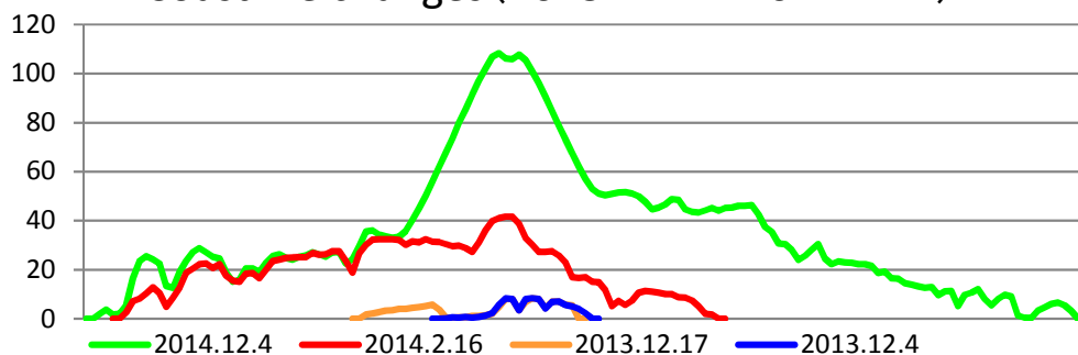
Cross-section view comparison at highest point around current crater (2013.12.4 ~ 2014.12.4)
