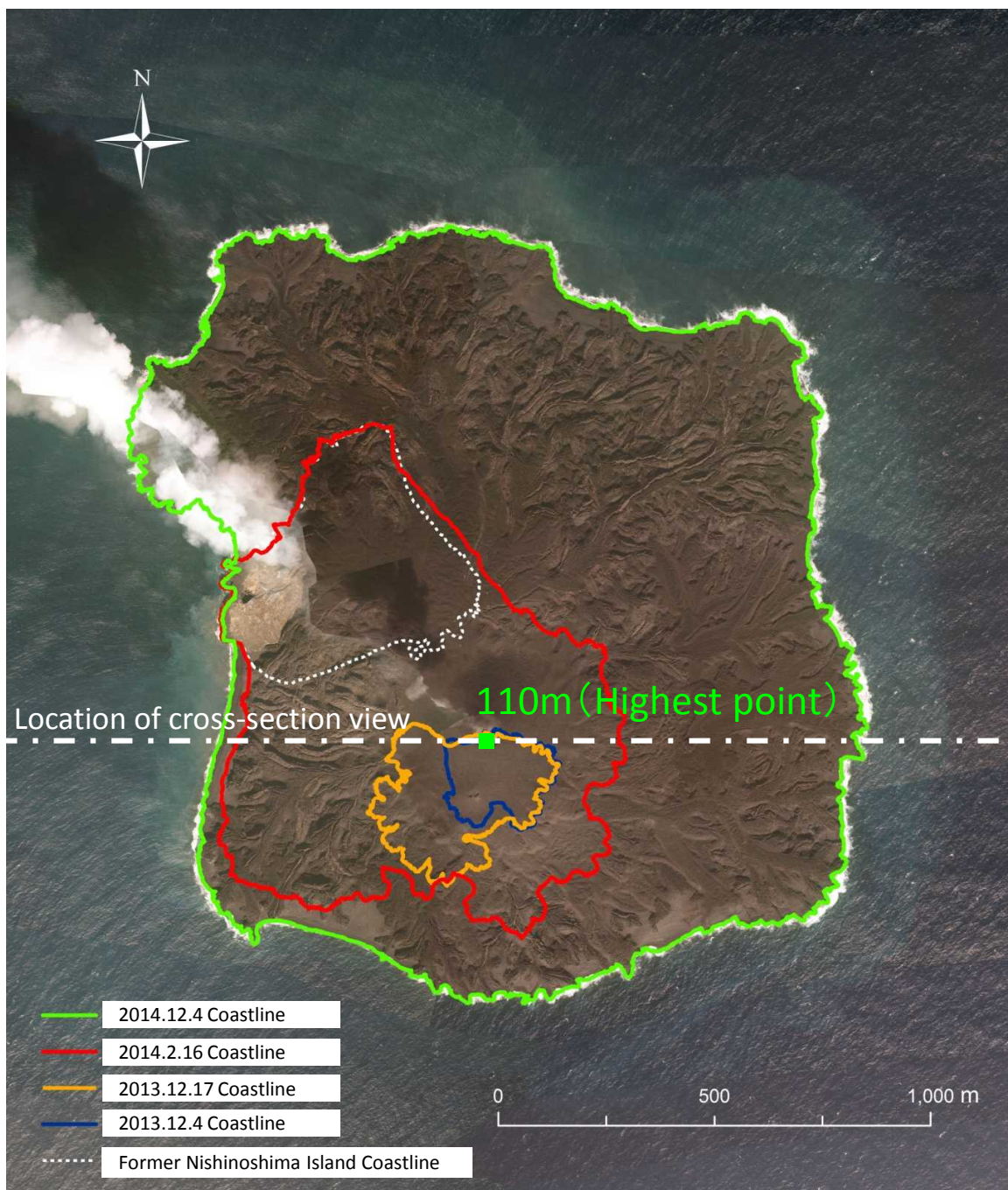
Coastline changes (2013.12.4 ~ 2014.12.4)
