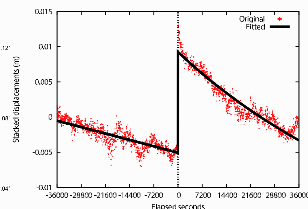
Fig. 11 Stacked kinematic GPS time series by considering offset polarity
