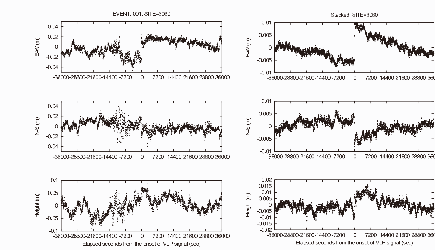
Fig. 7 (left) Time series for one event (right) Stacked time series
