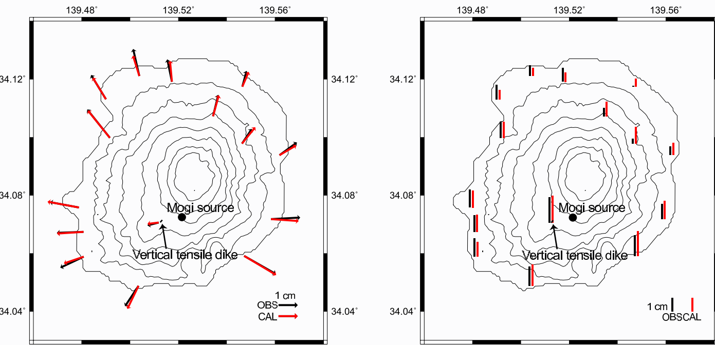
Fig. 9 Displacements associated with the VLP signals and the optimal source model
