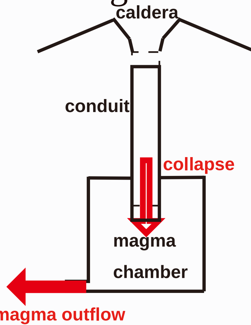
Fig. 5 Schematic diagram of “piston model” (after Kumagai et al., 2001)
