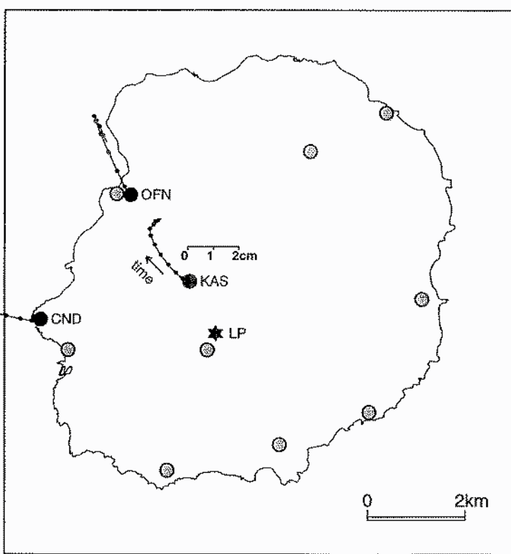
Fig. 4 Source location (from Kikuchi et al., 2001)
