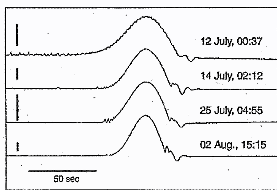
Fig. 3 Example of VLP signals (from Kumagai et al., 2001)
