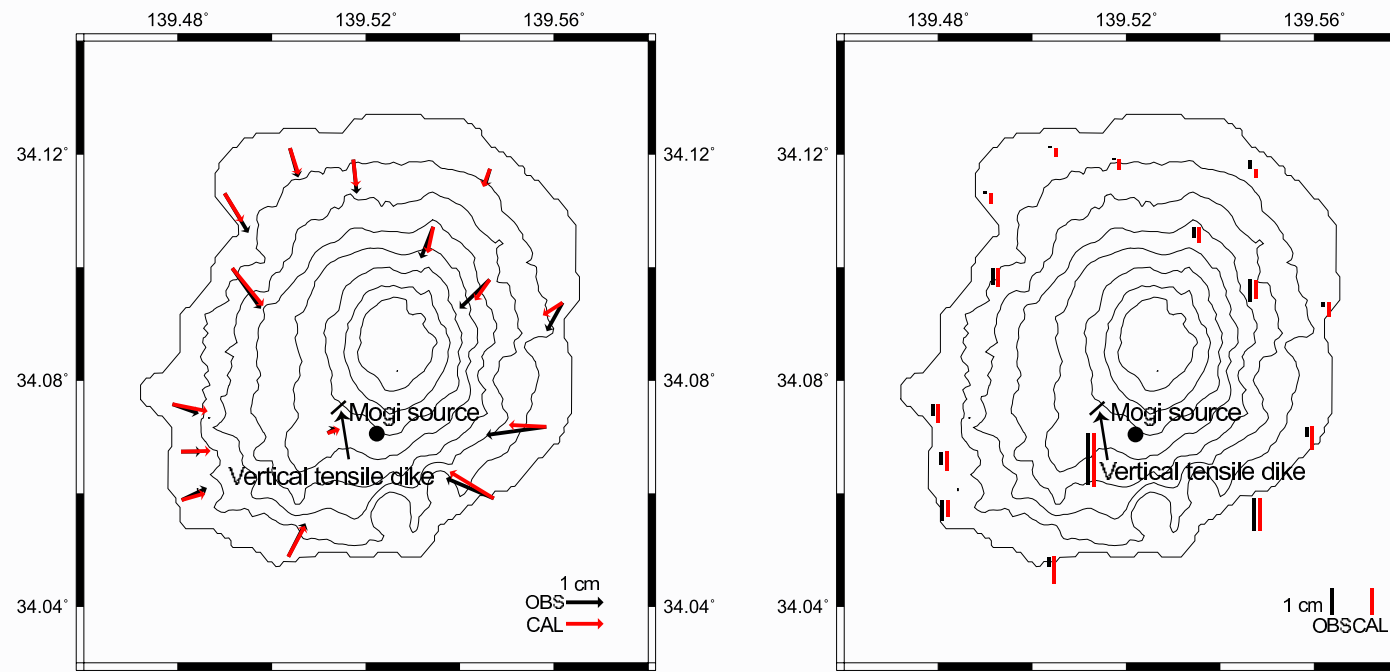
Fig. 10 Displacements associated with the linear trends and the optimal source model
