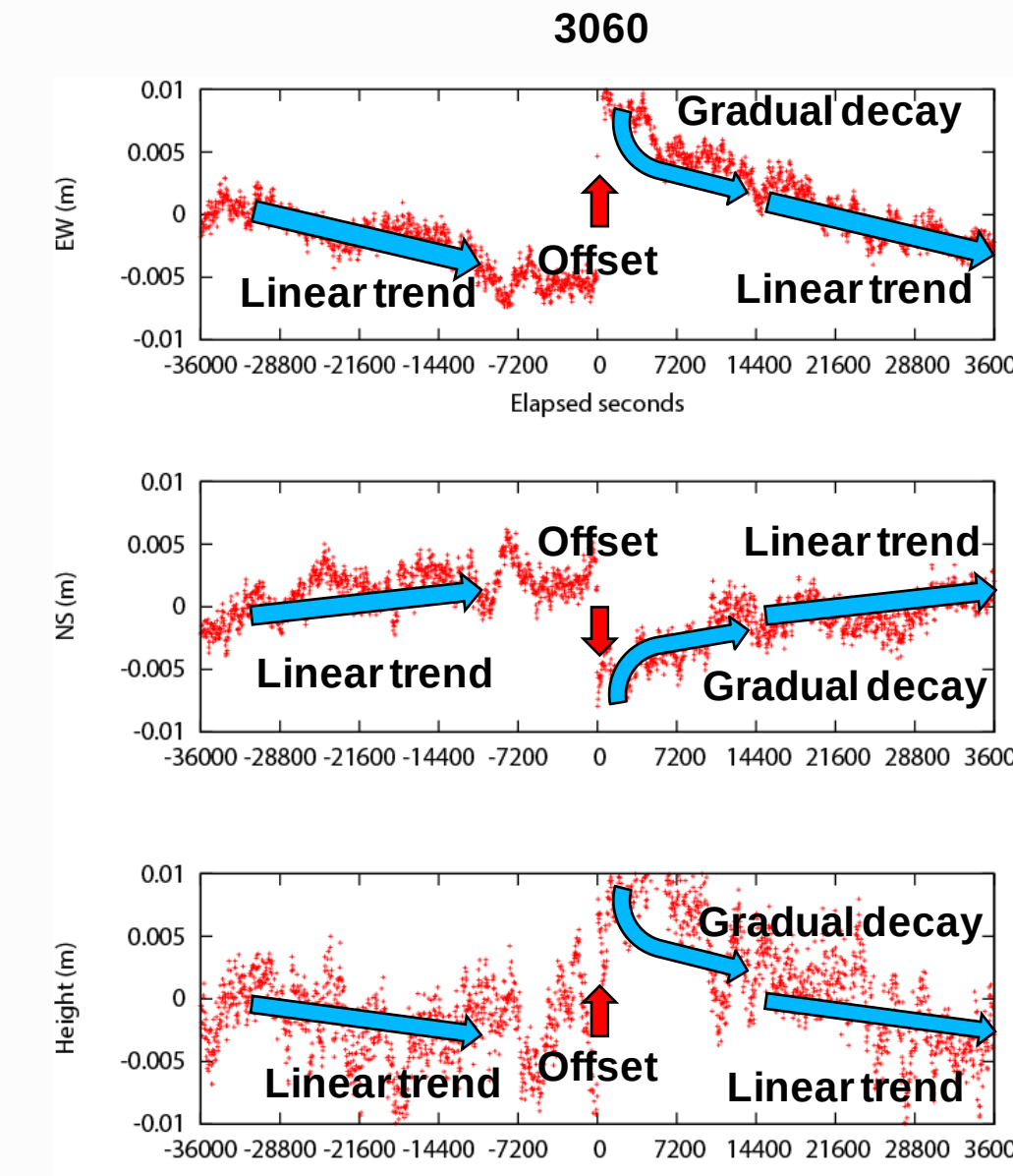
Fig. 8 Interpretation of time series
