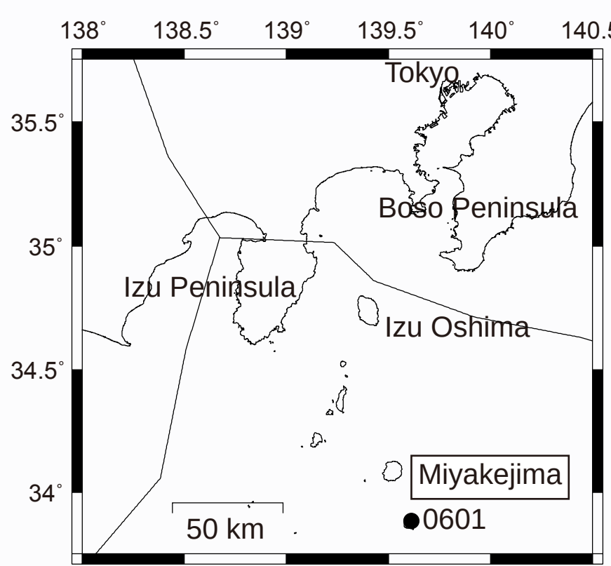
Fig. 1 Location of the Miyake-jima
