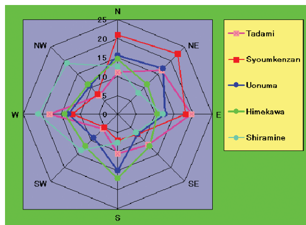
Fig. 8 Directions of avalanche furrows on slopes subject to full-depth snow avalanches locations are shown in Fig. 1.
