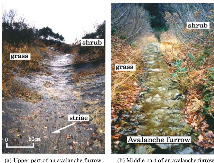
Fig. 6 Ground surface of the upper and middle part of an avalanche furrow in the Tadami area (November 1991, by the authors). Inclination is 40^\circ , and slope direction is southwest.
