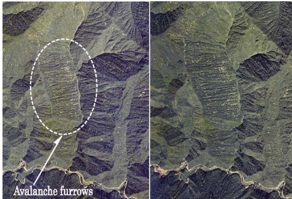
Fig. 4 Avalanche furrows in the Uonuma area; aerial photograph, taken during a snow-free period (September 1976, by the Geographical Survey Institute). Possible use stereo vision with 3D.
