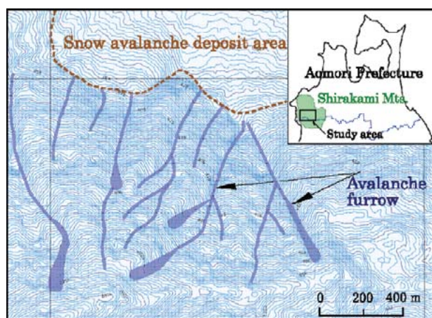
Fig. 18 Contour map using airborne laser scanning and avalanche furrows interpreted by contour map in Shirakami Mountains, Tohoku. Contour interval is 2 m.
