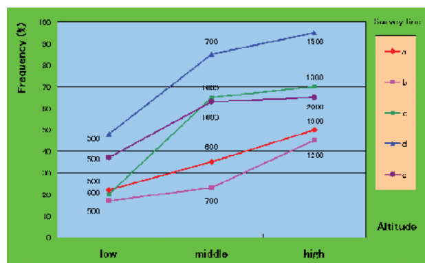
Fig. 11 Relationship between the occurrence of avalanche furrows and altitude. The survey lines are shown in Fig.10. a : Hokkaido, b : Northern Tohoku c : Southern Tohoku d : Eastern Hokuriku e : Western Hokuriku. The altitudes are classified into mountains of low, middle and high for each survey line. The representative altitudes (m) for the classes are indicated.
