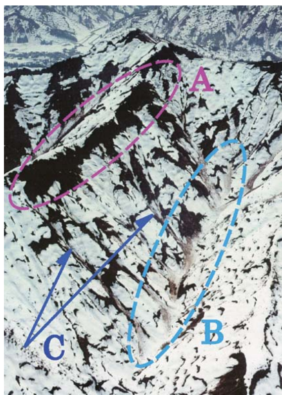
Fig. 2 Aerial photograph of slopes subjected to full-depth snow avalanches in Uonuma area. A : FDSA starting area B : avalanche deposit area C : avalanche furrow (March 1989, by the Geographical Survey Institute).
