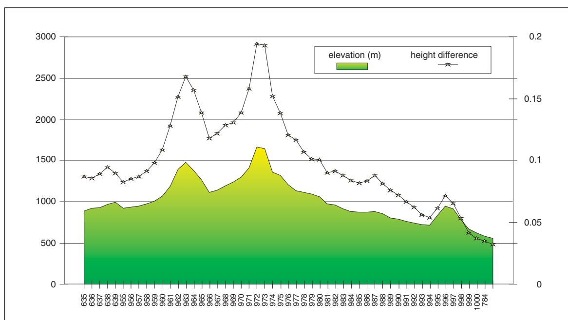
Fig. 10 Difference between orthometric height and normal orthometric height along the leveling route through Nomugi Pass
