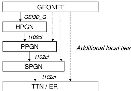
Fig. 3 Sequence of network adjustments. The upper level of the network is fixed in each network adjustment. GS13D_G and t102ci are the programs used for the adjustments (See Section 3.4.3).
